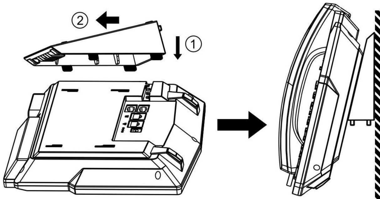
Figure 3 - Wall-mount Installation
